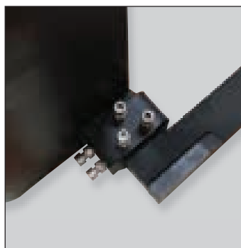
NAS and AS Models feature adjustable straddle bases with inside dimension of 40" to 50" and forged forks.
